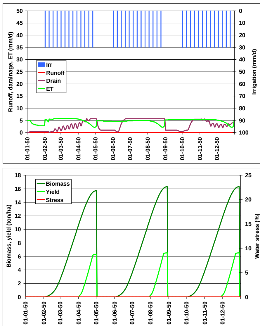
Figure 24. Output AquaCrop for the adaptation to change from two to three growing seasons: soil water (top) and crop growth (bottom).
