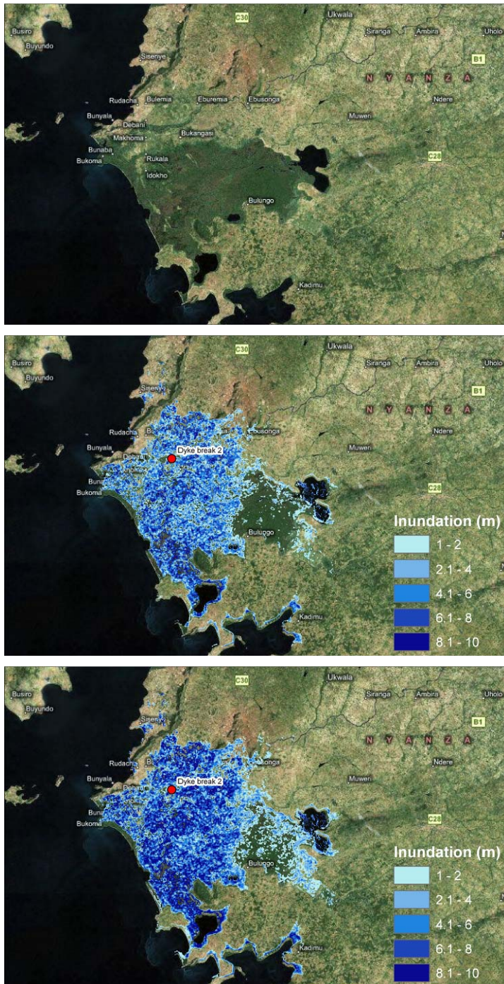
Figure 17 Estimate flood depth for a recurrence time of 5 years for the current climate (middle maps) and the 2050 climate (bottom map). The top figure shows an overview of the area.
