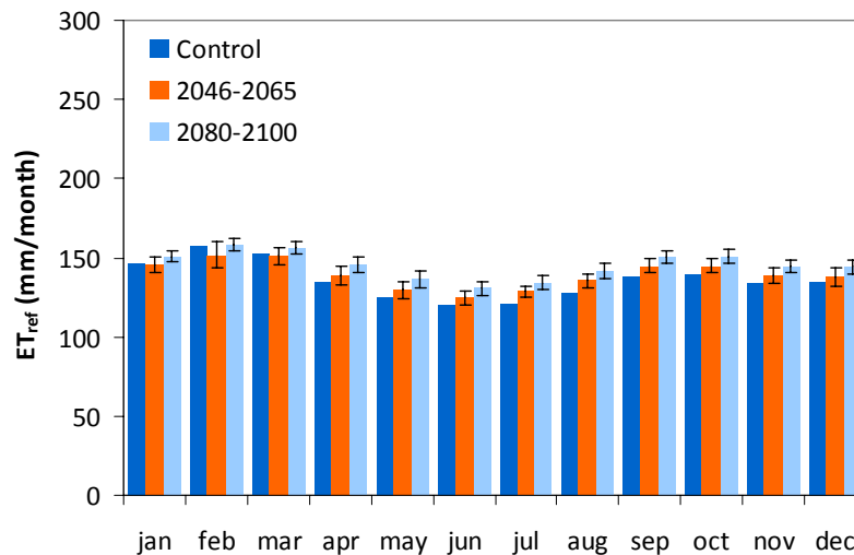
Figure 10 Projected monthly changes in reference evapotranspiration (Hargreaves) for Kakamega. The control period is 1960-1990. The future projections are the multi-model average (MMA) of 6 GCMs. The error bars denote +/- one standard deviation between the 6 GCMs.
