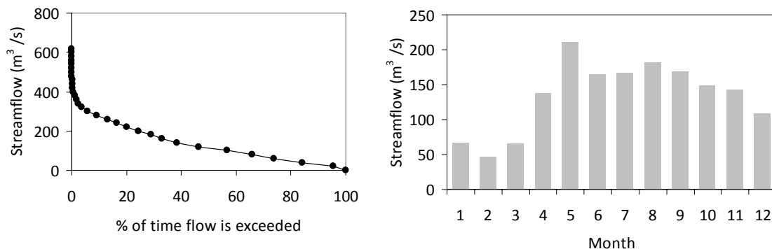
Figure 13: Flow duration curve and mean monthly discharge based on daily discharge data from 1985-2006
